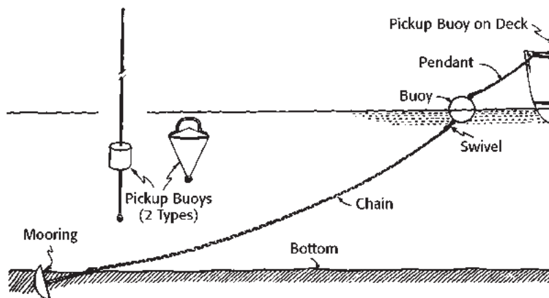
Mooring Tackle
